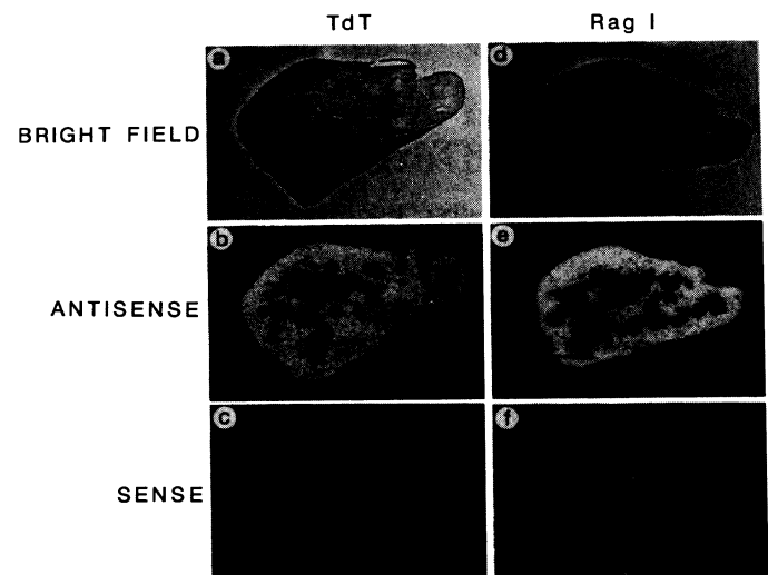
FIG. 1. Location of TdT and RAG-1 transcripts in thymus sections from a 12-day-old mouse. Thymus sections were hybridized with TdT and RAG-1 RNA probes, as described, and stained with toluidine blue. Sections hybridized with antisense probes were photographed by using both bright-field (a and d) and dark-field (b and e) optics at \times 17.5 . Serial sections hybridized with sense probes (c and f) were photographed at the same magnification using dark-field optics.
