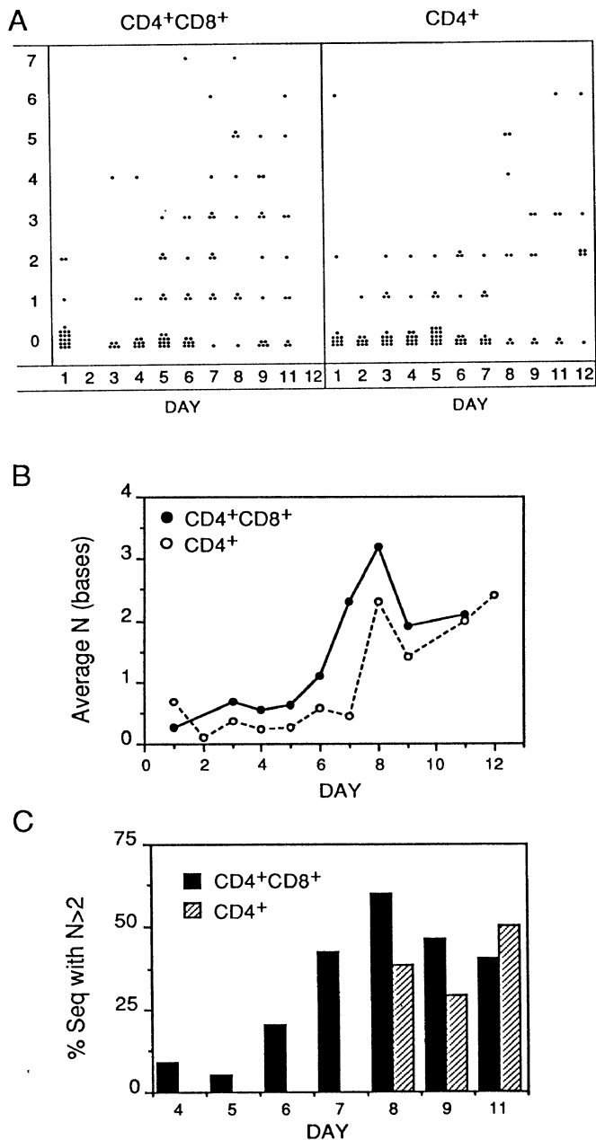
FIG. 4. Time course of N nucleotide addition. N additions to V_{\beta 6}^{+} TCRs from CD4^{+}CD8^{+} and CD4^{+}CD8^{-} thymocytes from postnatal mice. V_{\beta 6}^{+} sequences were obtained from sorted cells from developmentally staged B6D2 mice. Nucleotides were assigned to V, D, and J segments that compose the junctional region, as described (16). Mono- or dinucleotides representing inverted repeats of undigested germ-line termini were grouped as P nucleotides (10). Remaining nucleotides that could not be assigned to one of the above categories were considered template-independent additions and were, thus, designated N nucleotides. (A) Each dot represents one sequence, the position along the y axis indicating the number of N nucleotides in that sequence, and the x axis indicating the day after birth the sample was taken. Repeats are represented only once; the few out-of-frame sequences obtained are omitted. (B) Average number of N nucleotides per sequence. Averages were determined from the data in A. (C) Percentage of sequences (Seq) with >2 N nucleotides per sequence. Percentages were determined from the data in A.
