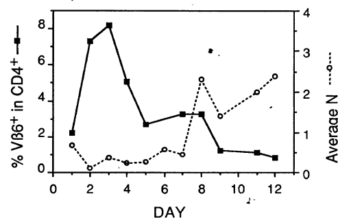
FIG. 5. Comparison of timing of clonal deletion of V_{\beta 6}^{+} CD4^{+} T cells and of amplification of N-region diversity in V_{\beta 6}^{+} TCRs. ■, Proportion of V_{\beta 6}^{+} CD4^{+}CD8^{-} cells expressed as percentage of total CD4^{+} cells; ○, average number of N nucleotides (sequence data of Fig. 4 are superimposed for clarity).
