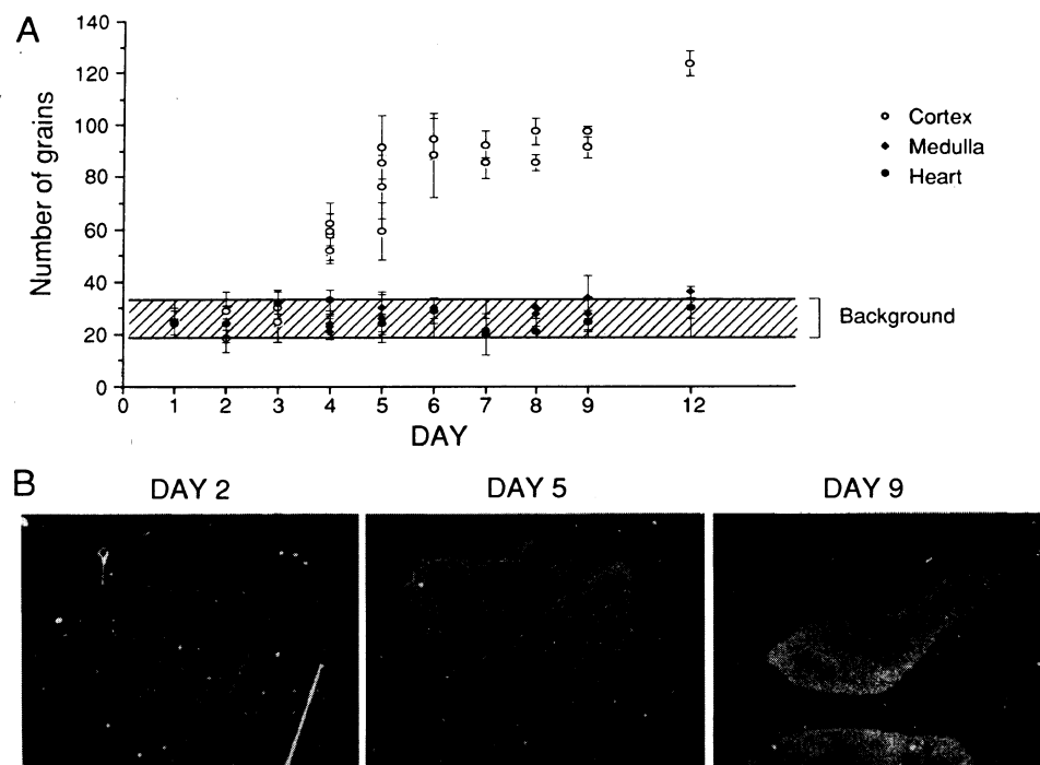
FIG. 3. Timing of onset of TdT expression in the thymus. (A) Grain counts. Sections from thymi taken from newborn mice at the days indicated (day of birth designated day 1) were hybridized with an antisense TdT RNA probe. Silver grains were counted to assess specificity and relative levels of hybridization. Each symbol represents the average number of grains in an equal area of tissue (thymic cortex, thymic medulla, and heart), and the shaded region indicates the number in an equal area of slide (background); grains in three to nine distinct areas of each region were counted. (B) Dark-field photographs ( \times 17.5 ) of representative sections used for the grain counts in A.
